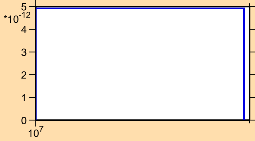
\sigma vs. E for ^{102}\text{Ag} (mt 34)
