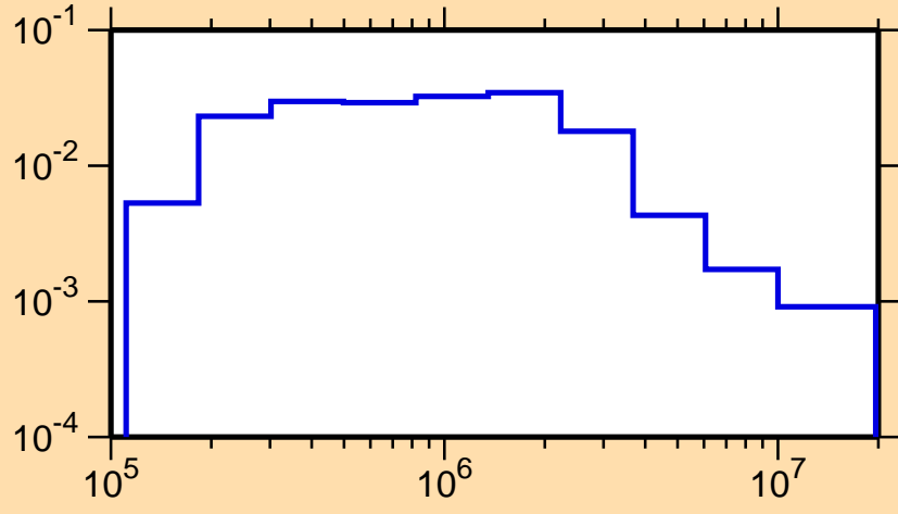
\sigma vs. E for ^{102}\text{Ag}(n,n_3)
