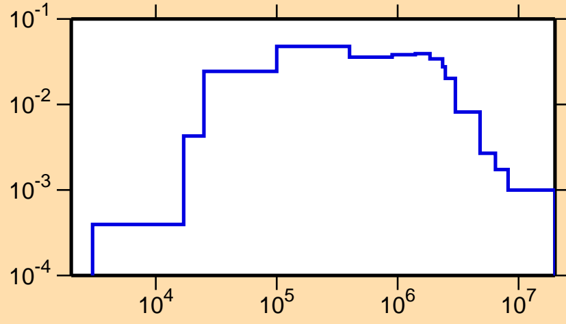
\sigma vs. E for ^{102}\text{Ag}(n,n_1)
