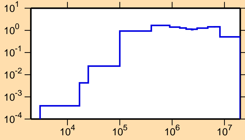
\sigma vs. E for ^{102}\text{Ag}(n,\text{inel.})
