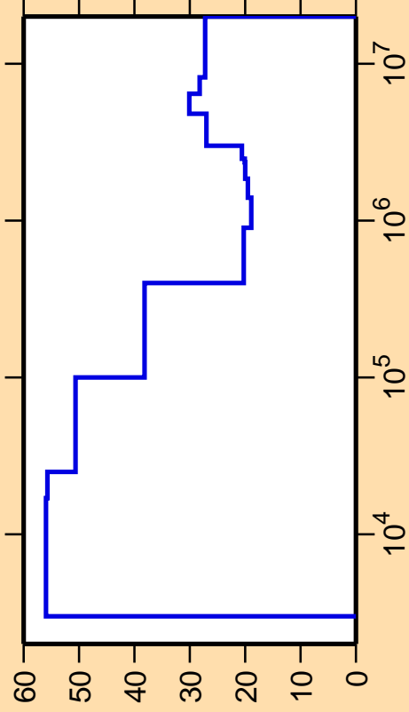
\Delta\sigma/\sigma vs. E for ^{102}\text{Ag}(n,n_1)
