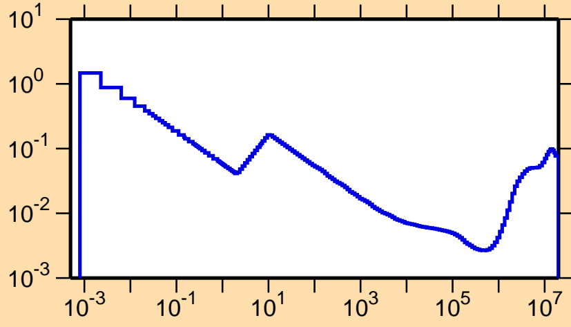
\sigma vs. E for ^{102}\text{Ag}(n,\alpha)
