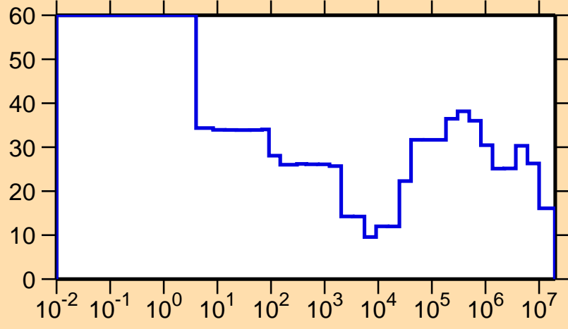
\Delta\sigma/\sigma vs. E for ^{102}\text{Ag}(n,p)
