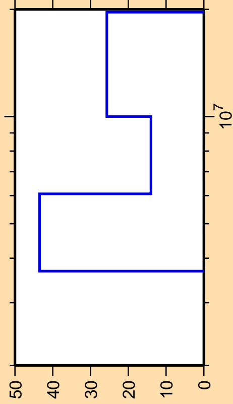
\Delta\sigma/\sigma vs. E for ^{102}\text{Ag}(n,np)
