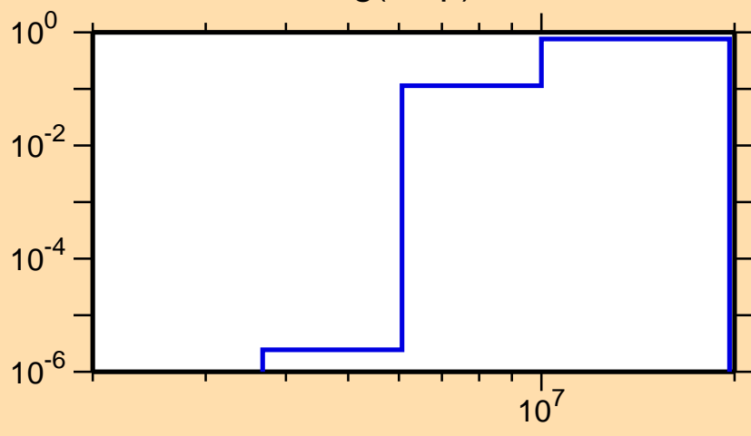
\sigma vs. E for ^{102}\text{Ag}(n,np)
