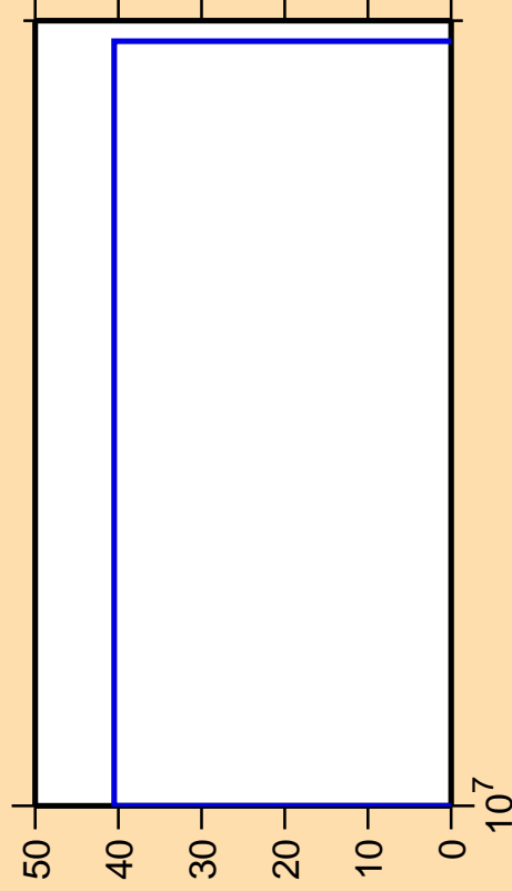
\Delta\sigma/\sigma vs. E for ^{102}\text{Ag} (mt 34)
