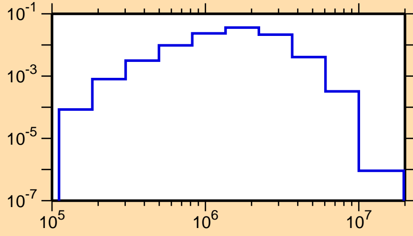
\sigma vs. E for ^{102}\text{Ag}(n,n_4)
