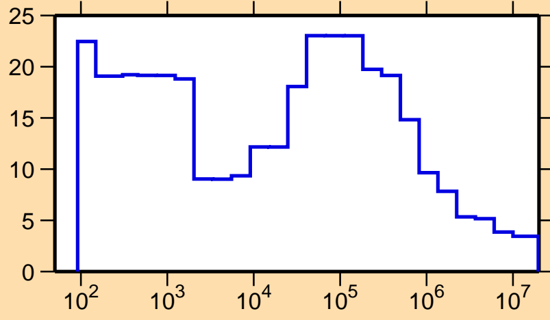
\Delta\sigma/\sigma vs. E for ^{102}\text{Ag}(n,\text{nonel.})
