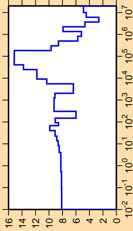
\Delta\sigma/\sigma vs. E for ^{103}\text{Ag}(n,\text{el.})
