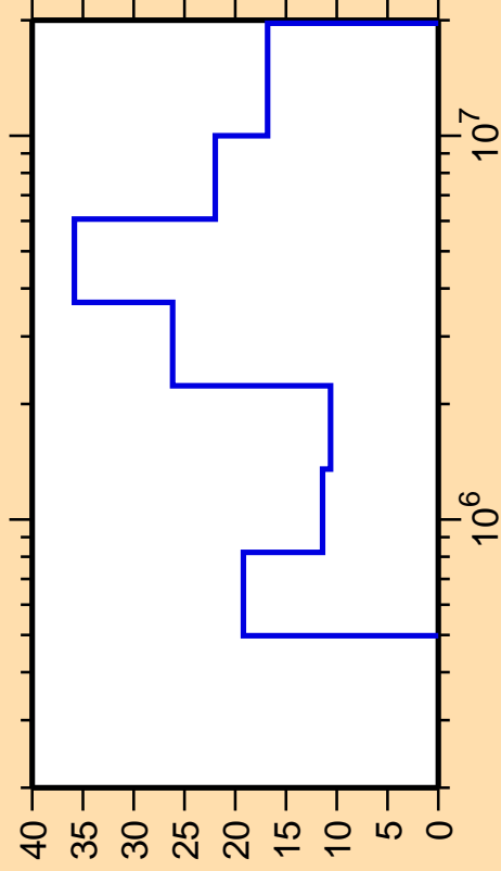
\Delta\sigma/\sigma vs. E for ^{103}\text{Ag}(n,n_4)
