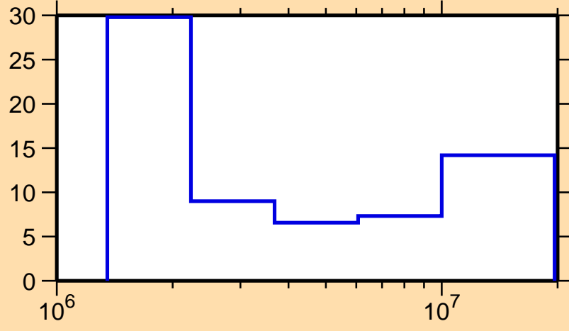
\Delta\sigma/\sigma vs. E for ^{103}\text{Ag}(n,n\text{cont.})
