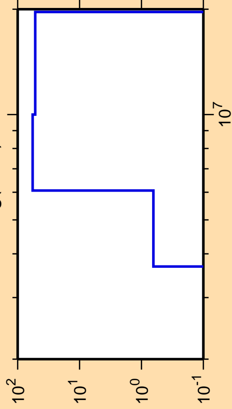
\Delta\sigma/\sigma vs. E for ^{103}\text{Ag}(n,n\alpha)
