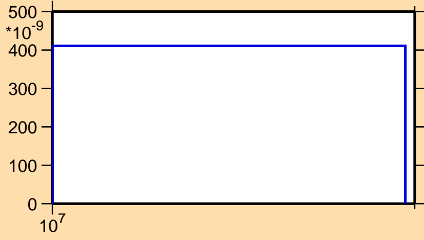
\sigma vs. E for ^{103}\text{Ag}(n,\text{nd})
