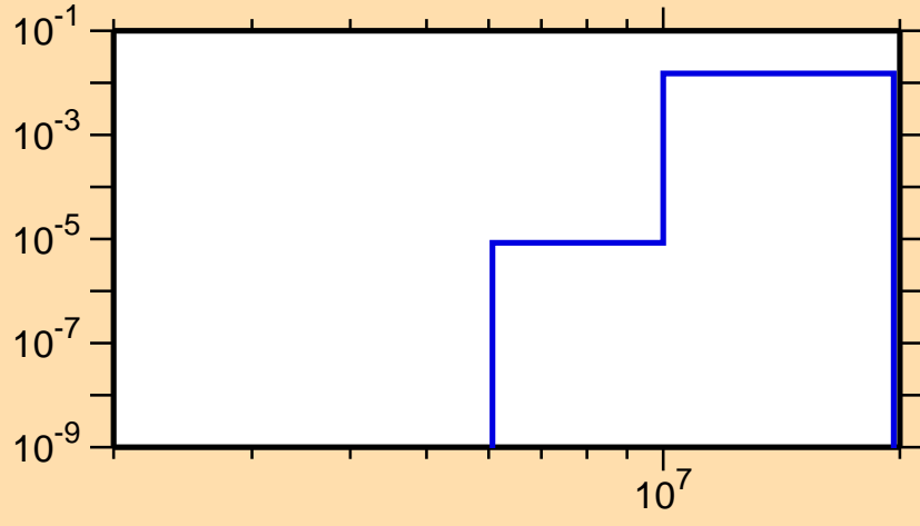
\sigma vs. E for ^{103}\text{Ag}(n,n\alpha)
