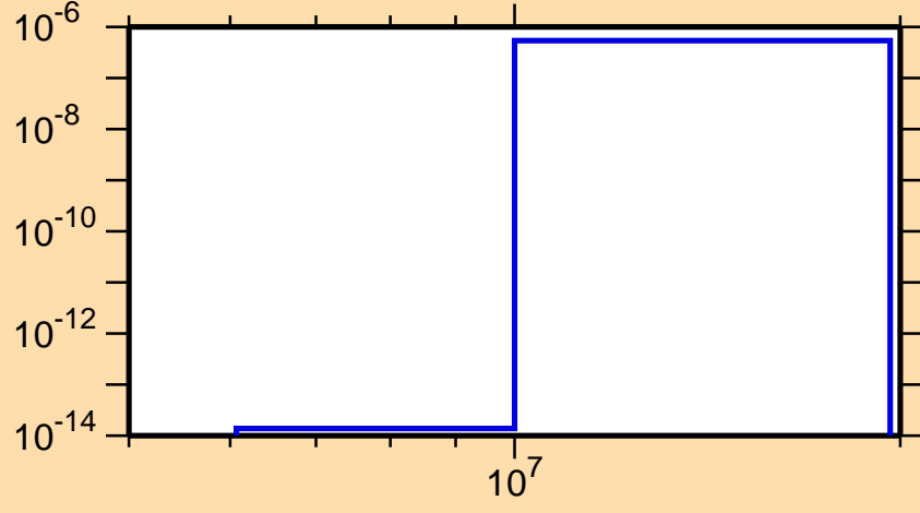
\sigma vs. E for ^{103}\text{Ag}(n,\text{He}3)
