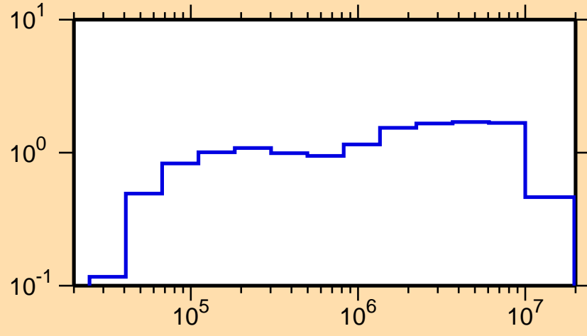
\sigma vs. E for ^{103}\text{Ag}(n,\text{inel.})
