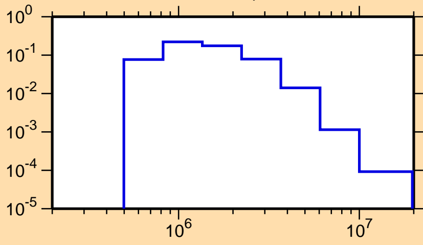
\sigma vs. E for ^{103}\text{Ag}(n,n_4)
