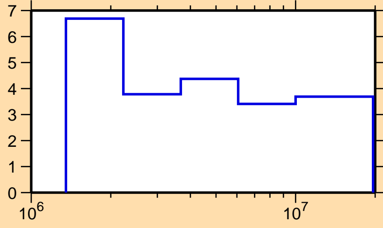
\Delta\sigma/\sigma vs. E for ^{103}\text{Ag}(n,\text{nonel.})
