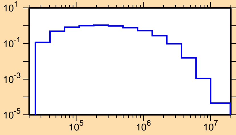
\sigma vs. E for ^{103}\text{Ag}(n,n_1)
