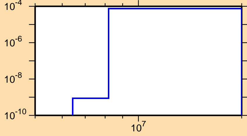
\sigma vs. E for ^{103}\text{Ag}(n,p\alpha)
