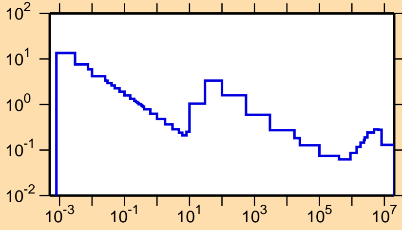
\sigma vs. E for ^{103}\text{Ag}(n,p)
