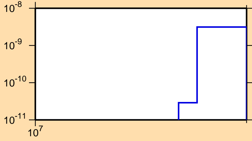
\sigma vs. E for ^{105}\text{Ag}(\text{mt } 45)
