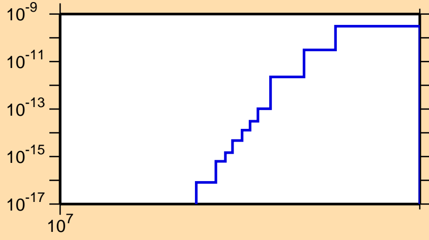
\sigma vs. E for ^{105}\text{Ag}(\text{mt117})
