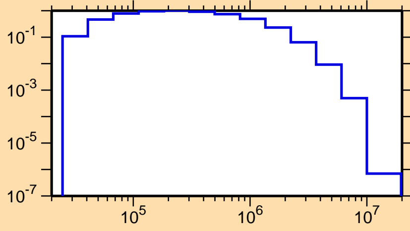
\sigma vs. E for ^{105}\text{Ag}(n,n_2)
