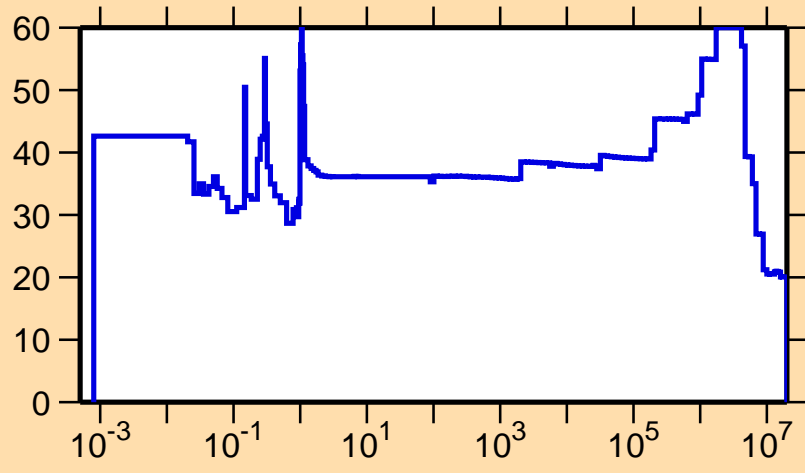
\Delta\sigma/\sigma vs. E for ^{106}\text{Ag}(n,p)
