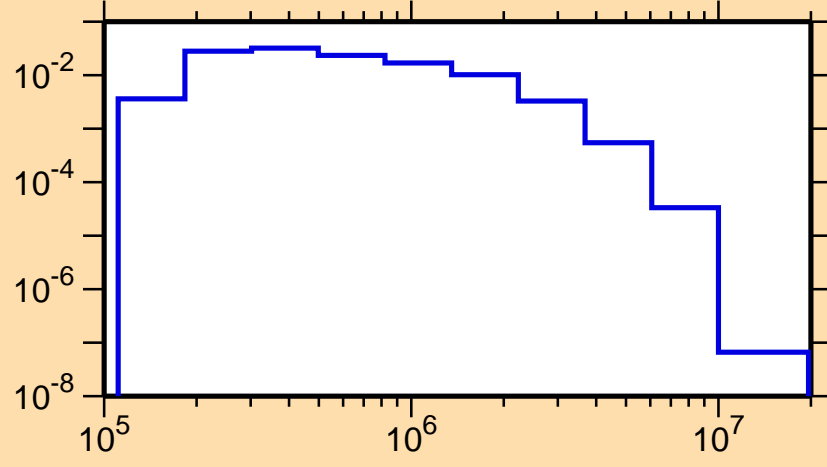
\sigma vs. E for ^{106}\text{Ag}(n,n_4)
