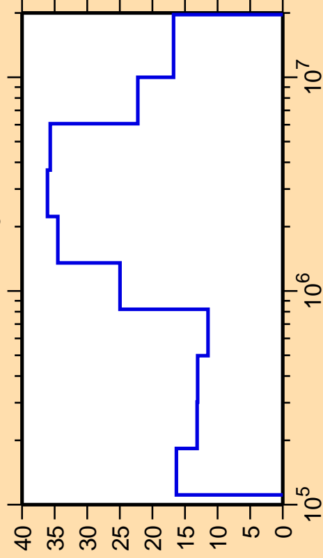
\Delta\sigma/\sigma vs. E for ^{106}\text{Ag}(n,n_3)
