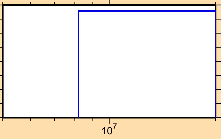
\sigma vs. E for ^{106}\text{Ag}(\text{mt117})
