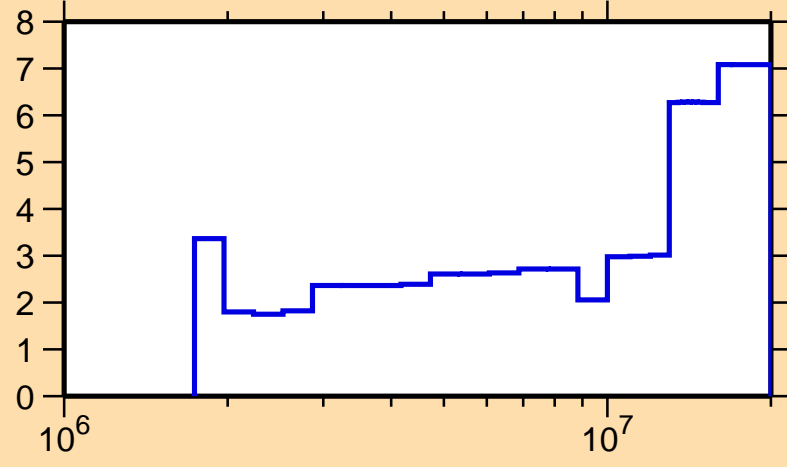
\Delta\sigma/\sigma vs. E for ^{107}\text{Ag}(n,n\text{cont.})
