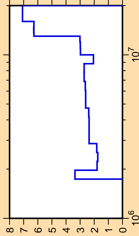
\Delta\sigma/\sigma vs. E for ^{107}\text{Ag}(n,n\text{cont.})
