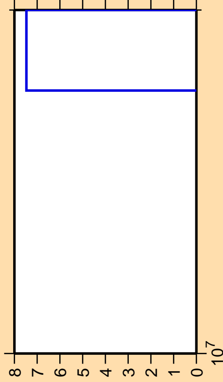
\Delta\sigma/\sigma vs. E for ^{107}\text{Ag}(n,3n)
