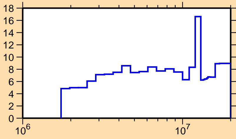
\Delta\sigma/\sigma vs. E for ^{107}\text{Ag}(n, n_1)
