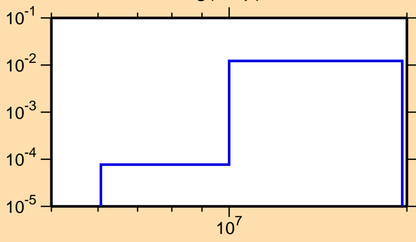
\sigma vs. E for ^{107}\text{Ag}(n,np)
