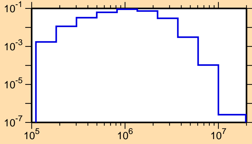
\sigma vs. E for ^{107}\text{Ag}(n,n_2)
