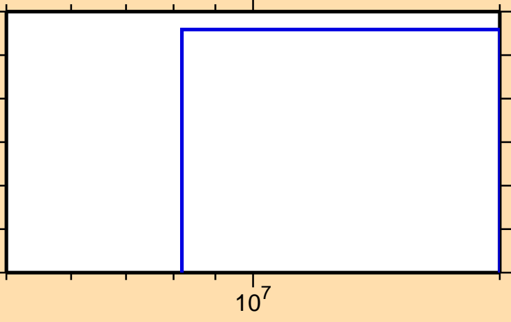
\sigma vs. E for ^{108}\text{Ag}(n,\text{He}3)
