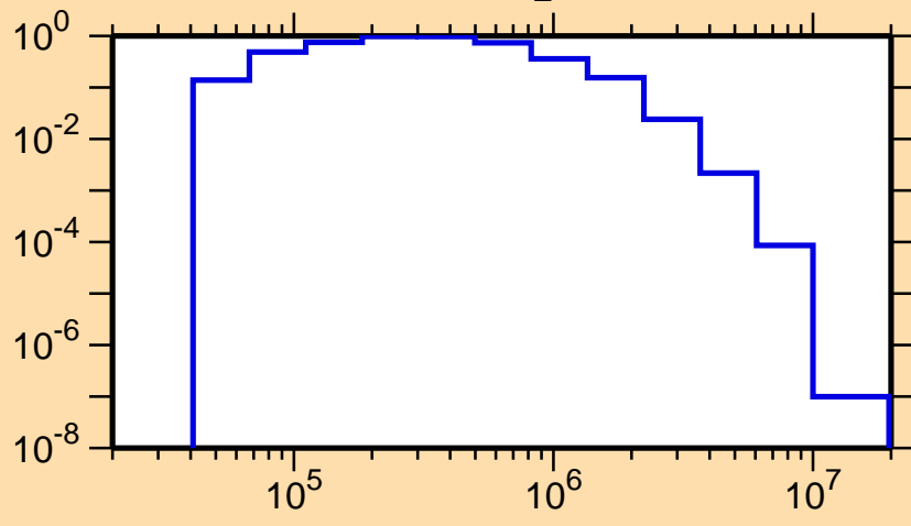
\sigma vs. E for ^{109}\text{Ag}(n,n_2)
