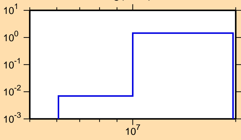
\sigma vs. E for ^{109}\text{Ag}(n,2n)
