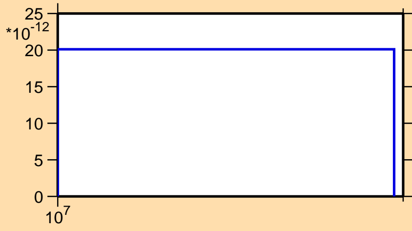
\sigma vs. E for ^{109}\text{Ag}(n,p\alpha)
