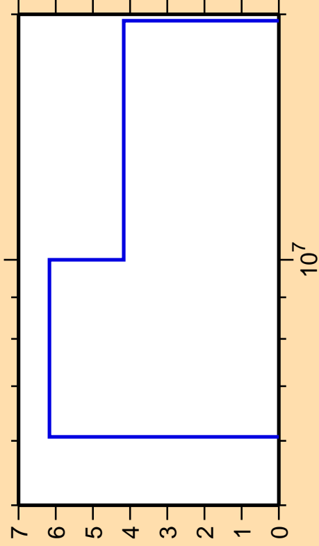
\Delta\sigma/\sigma vs. E for ^{109}\text{Ag}(n,2n)
