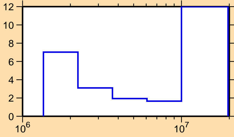
\Delta\sigma/\sigma vs. E for ^{109}\text{Ag}(n,n\text{cont.})
