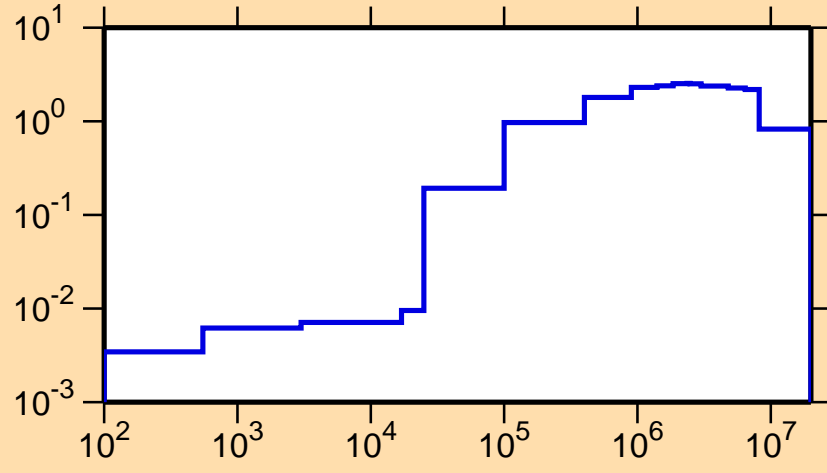
\sigma vs. E for ^{109}\text{Ag}(n,\text{inel.})
