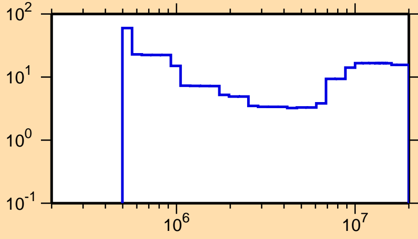
\Delta\sigma/\sigma vs. E for ^{110}\text{Ag}(n,n\text{cont.})
