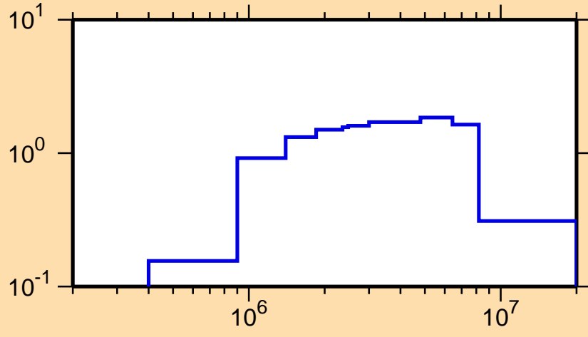
\sigma vs. E for ^{110}\text{Ag}(n,n\text{cont.})
