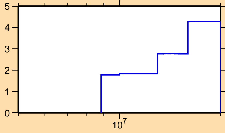
\Delta\sigma/\sigma vs. E for ^{111}\text{Ag}(n,\text{el.})
