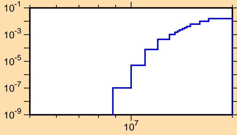
\sigma vs. E for ^{111}\text{Ag}(n,np)
