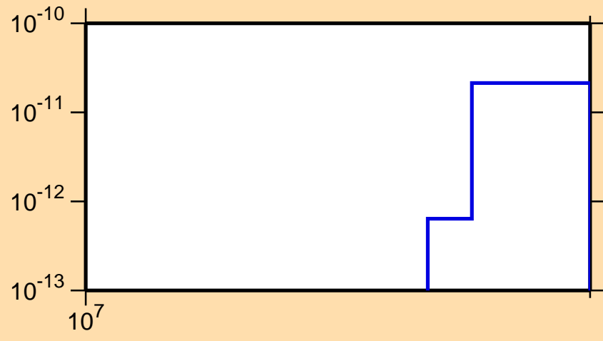
\sigma vs. E for ^{111}\text{Ag}(n,p\alpha)
