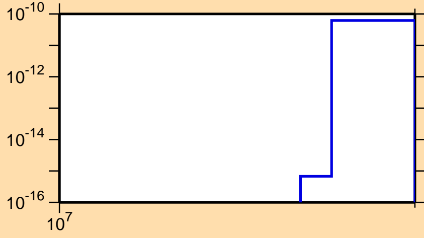
\sigma vs. E for ^{111}\text{Ag}(n,2n\alpha)
