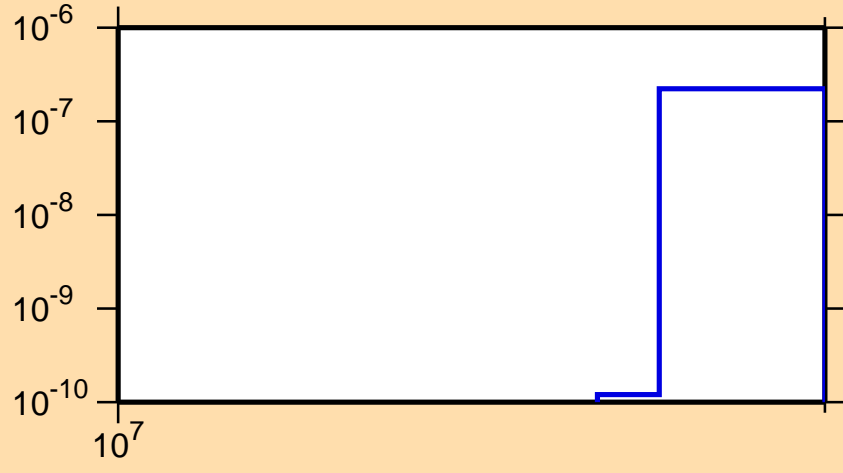
\sigma vs. E for ^{111}\text{Ag}(n,nt)
