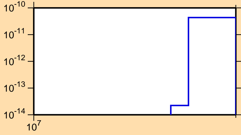
\sigma vs. E for ^{111}\text{Ag}(n,\text{He}3)
