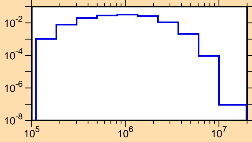
\sigma vs. E for ^{111}\text{Ag}(n,n_2)
