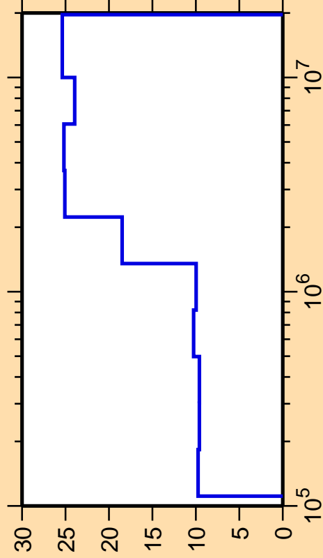
\Delta\sigma/\sigma vs. E for ^{111}\text{Ag}(n,n_2)
