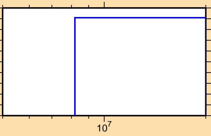
\sigma vs. E for ^{111}\text{Ag}(n,t)
