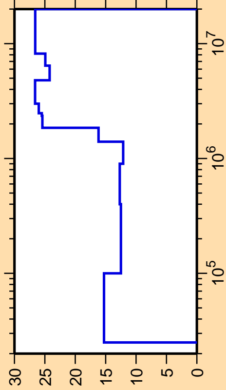
\Delta\sigma/\sigma vs. E for ^{111}\text{Ag}(n,n_1)
