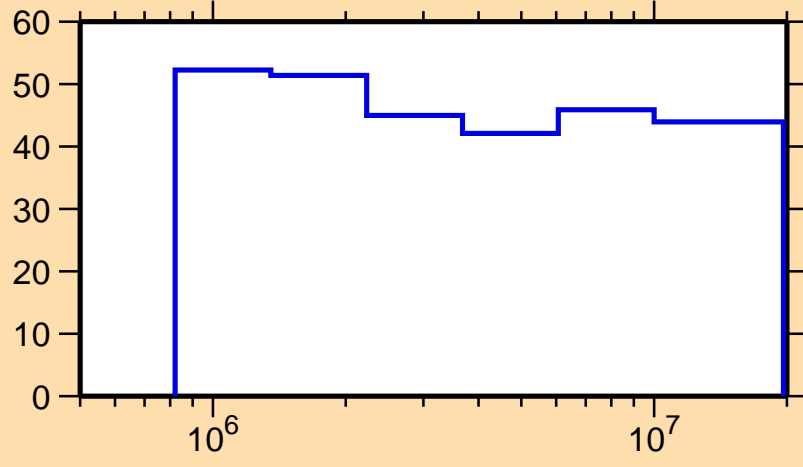
\Delta\sigma/\sigma vs. E for ^{112}\text{Ag}(n,p)
