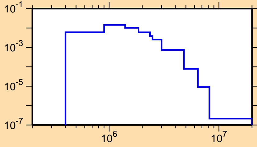
\sigma vs. E for ^{112}\text{Ag}(n,n_2)
