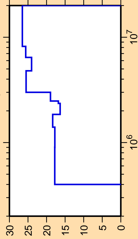
\Delta\sigma/\sigma vs. E for ^{112}\text{Ag}(n,n_3)
