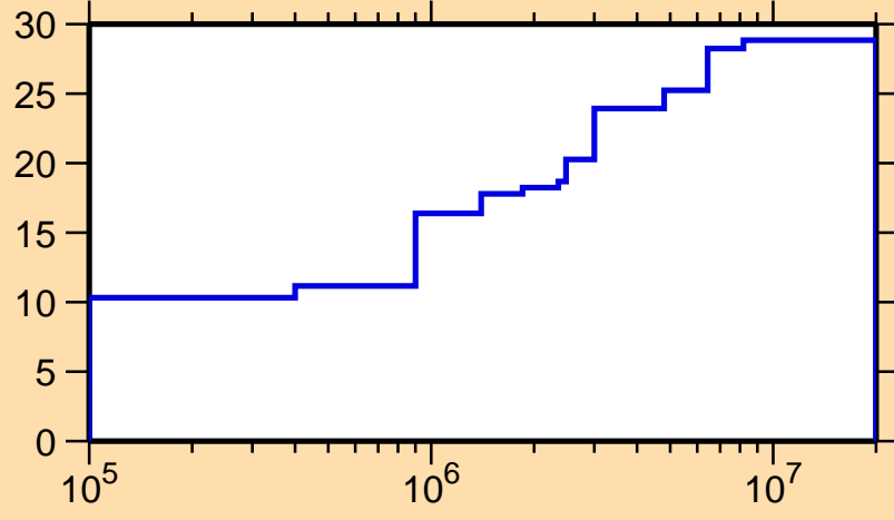
\Delta\sigma/\sigma vs. E for ^{112}\text{Ag}(n,n_1)
