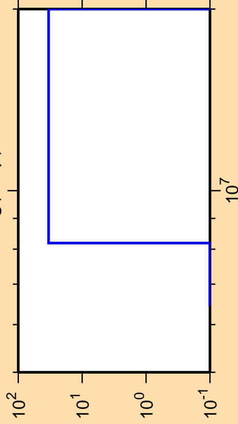
\Delta\sigma/\sigma vs. E for ^{112}\text{Ag}(n,np)
