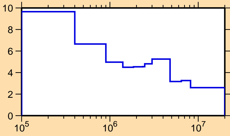
\Delta\sigma/\sigma vs. E for ^{112}\text{Ag}(n,\text{nonel.})
