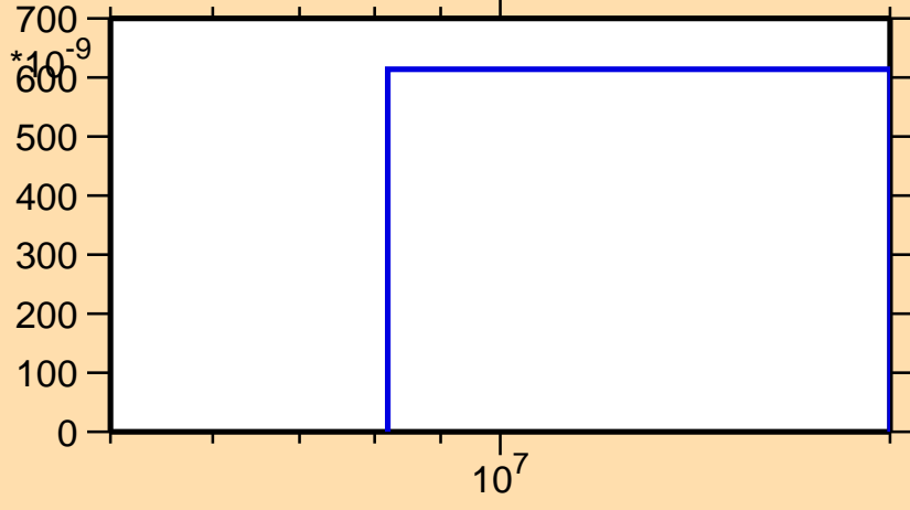
\sigma vs. E for ^{112}\text{Ag}(n,\text{nd})
