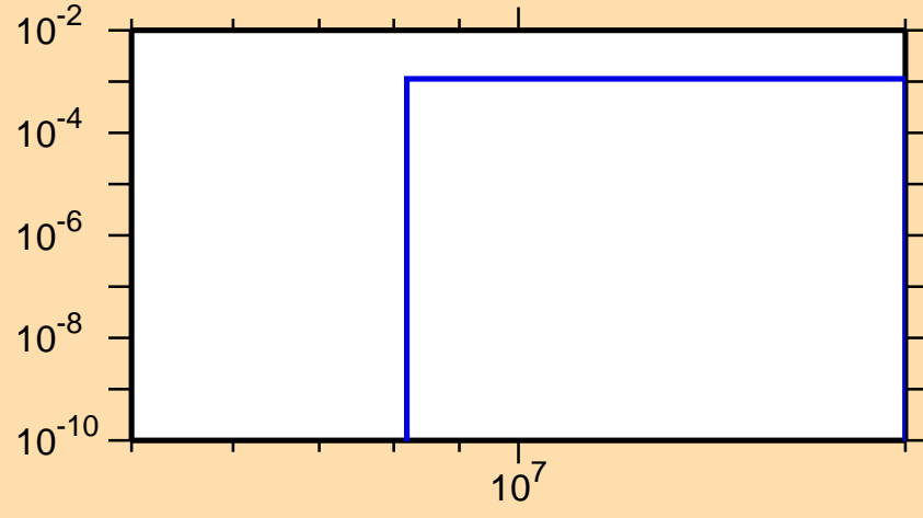
\sigma vs. E for ^{112}\text{Ag}(n,np)
