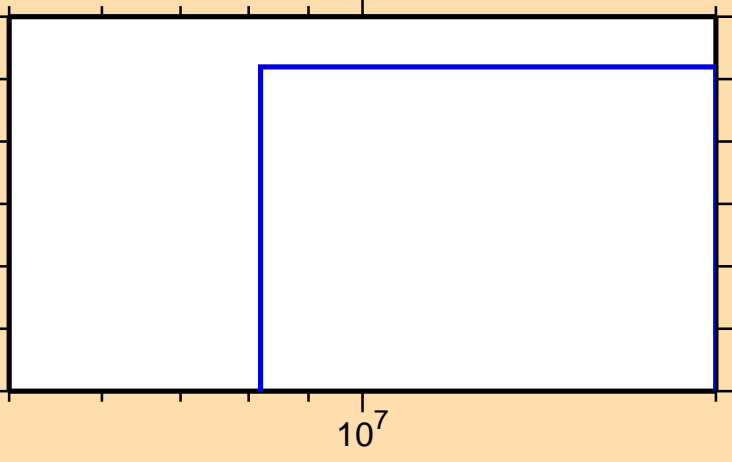
\sigma vs. E for ^{112}\text{Ag}(n,n\alpha)
