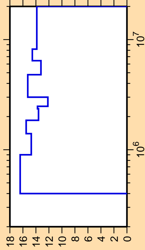
\Delta\sigma/\sigma vs. E for ^{112}\text{Ag}(n,n_4)
