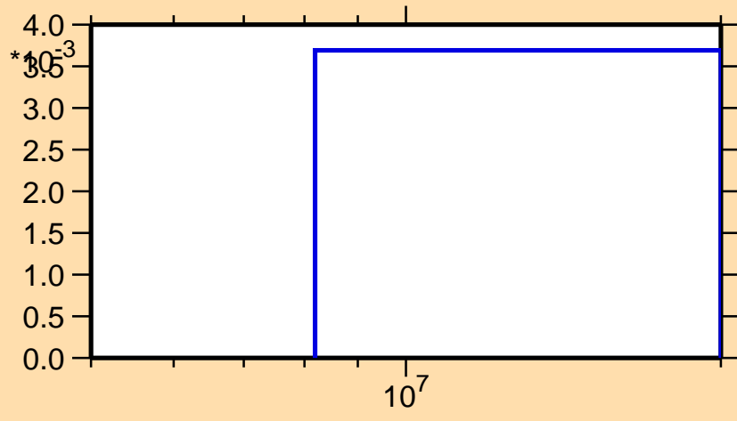
\sigma vs. E for ^{112}\text{Ag}(n,3n)
