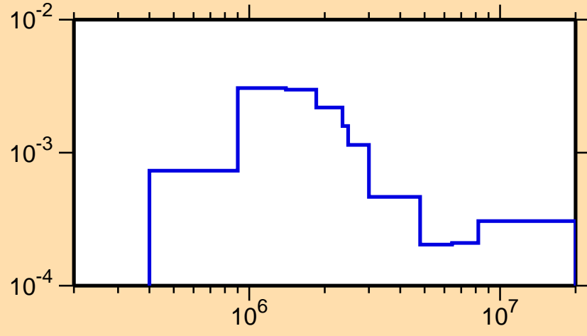
\sigma vs. E for ^{112}\text{Ag}(n,n_4)
