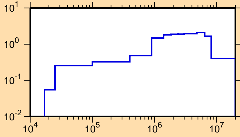
\sigma vs. E for ^{112}\text{Ag}(n,\text{inel.})
