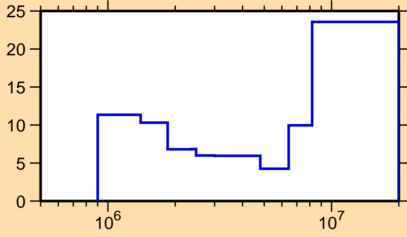
\Delta\sigma/\sigma vs. E for ^{112}\text{Ag}(n,n\text{cont.})
