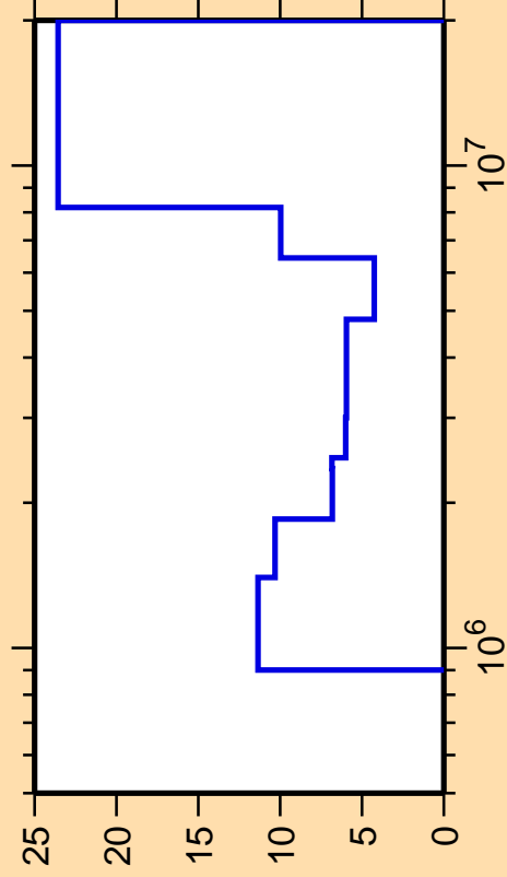
\Delta\sigma/\sigma vs. E for ^{112}\text{Ag}(n,n\text{cont.})
