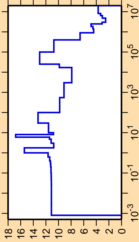
\Delta\sigma/\sigma vs. E for ^{112}\text{Ag}(n,\text{el.})
