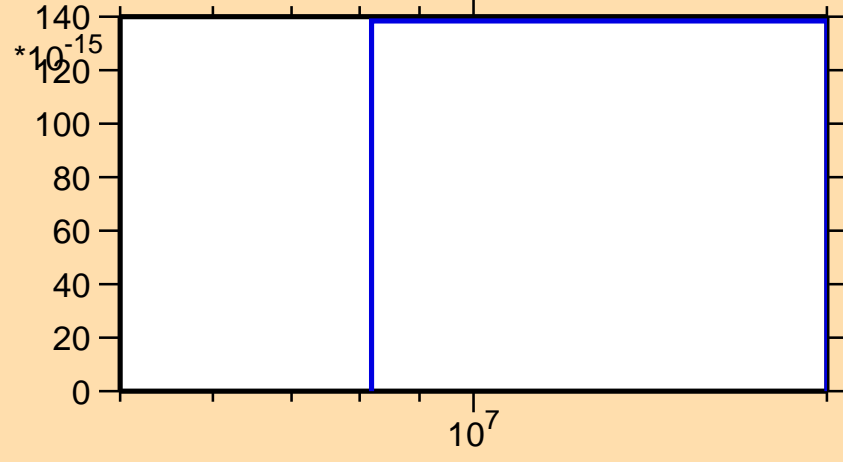
\sigma vs. E for ^{112}\text{Ag}(n,p\alpha)
