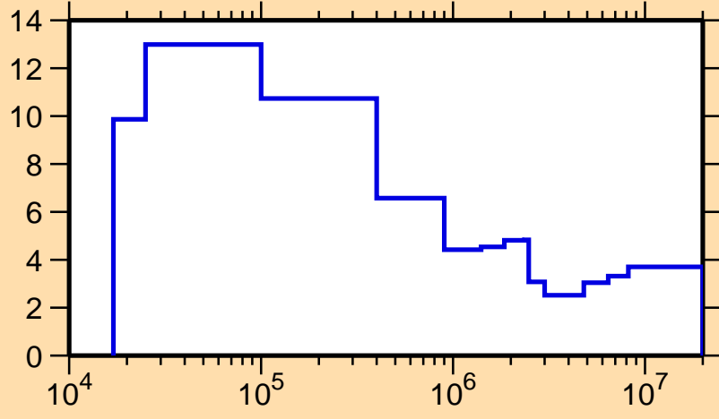
\Delta\sigma/\sigma vs. E for ^{112}\text{Ag}(n,\text{el.})
