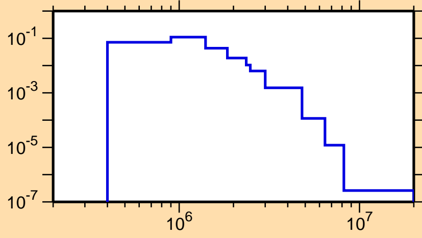
\sigma vs. E for ^{112}\text{Ag}(n,n_3)
