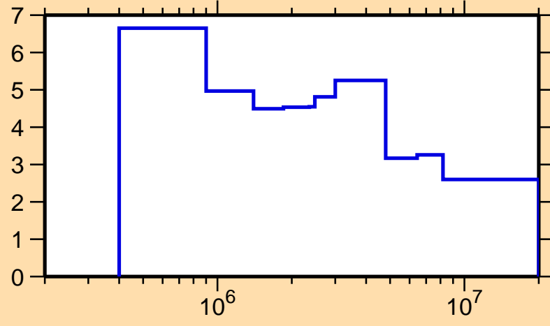
\Delta\sigma/\sigma vs. E for ^{112}\text{Ag}(n,\text{nonel.})
