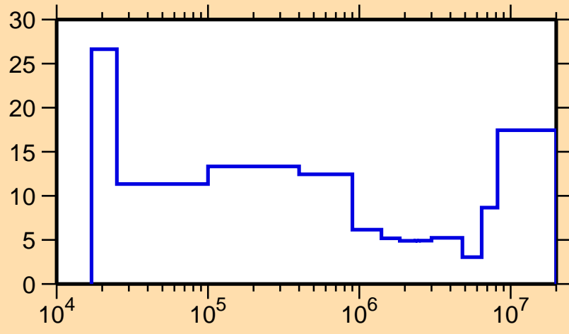
\Delta\sigma/\sigma vs. E for ^{112}\text{Ag}(n,\text{inel.})
