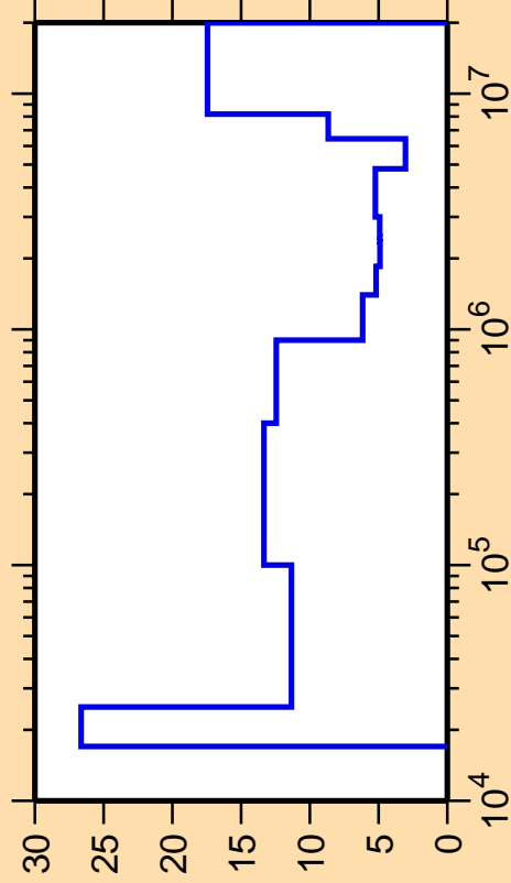
\Delta\sigma/\sigma vs. E for ^{112}\text{Ag}(n,\text{inel.})
