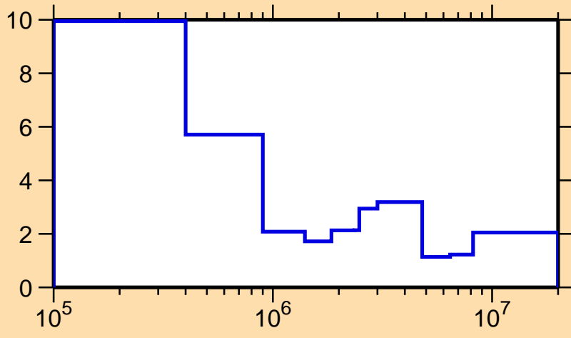
\Delta\sigma/\sigma vs. E for ^{112}\text{Ag}(n,\text{tot.})
