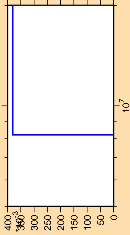
\Delta\sigma/\sigma vs. E for ^{112}\text{Ag}(n,p\alpha)
