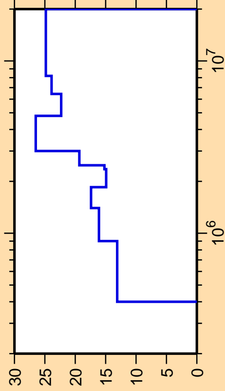
\Delta\sigma/\sigma vs. E for ^{112}\text{Ag}(n,n_2)
