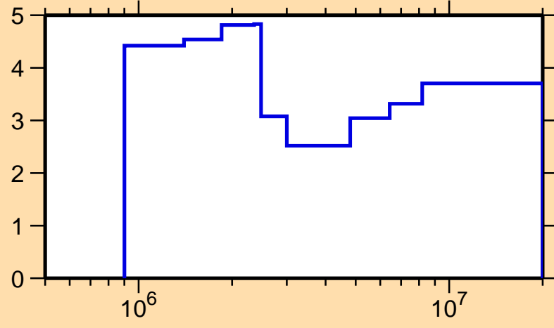
\Delta\sigma/\sigma vs. E for ^{112}\text{Ag}(n,\text{el.})
