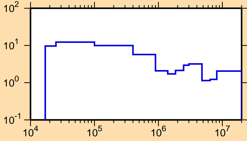
\Delta\sigma/\sigma vs. E for ^{112}\text{Ag}(n,\text{tot.})
