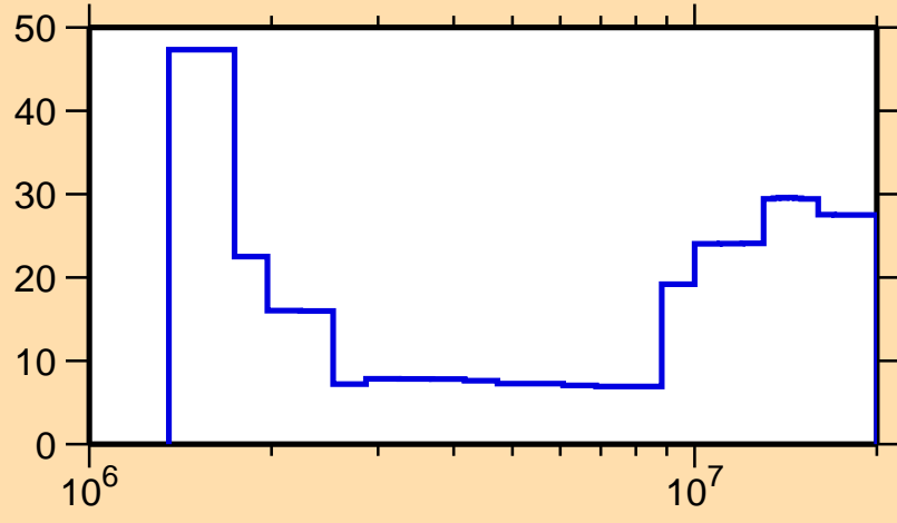
\Delta\sigma/\sigma vs. E for ^{113}\text{Ag}(n,n\text{cont.})
