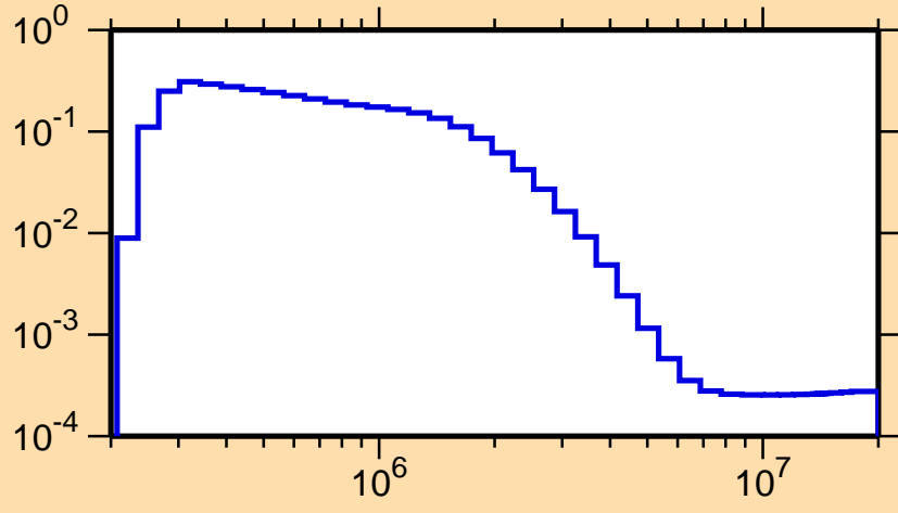
\sigma vs. E for ^{113}\text{Ag}(n,n_3)
