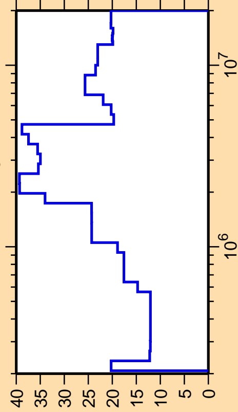
\Delta\sigma/\sigma vs. E for ^{113}\text{Ag}(n,n_3)
