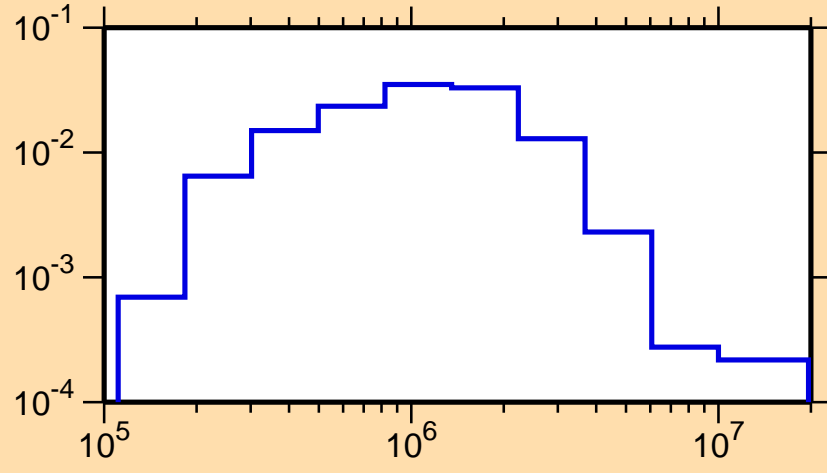
\sigma vs. E for ^{113}\text{Ag}(n,n_2)
