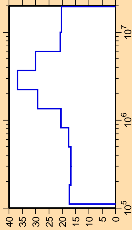
\Delta\sigma/\sigma vs. E for ^{113}\text{Ag}(n,n_2)
