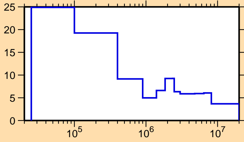
\Delta\sigma/\sigma vs. E for ^{113}\text{Ag}(n,\text{el.})
