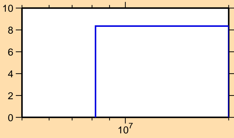
\Delta\sigma/\sigma vs. E for ^{113}\text{Ag}(n,2n)
