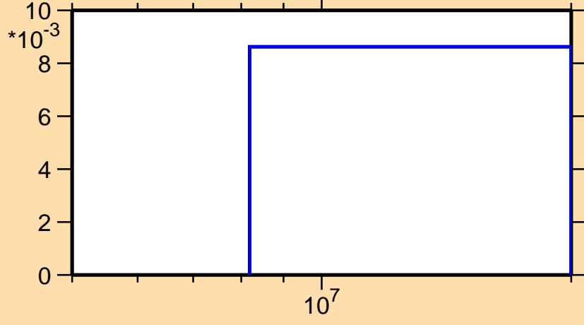
\sigma vs. E for ^{113}\text{Ag}(n,3n)
