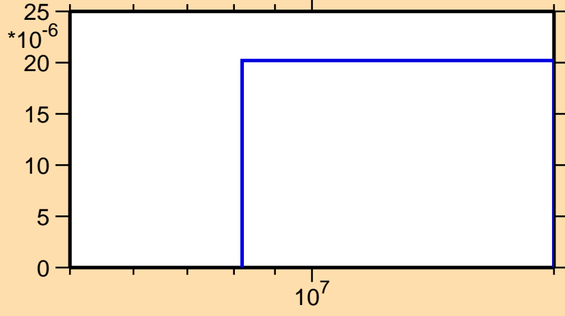
\sigma vs. E for ^{113}\text{Ag}(n,n\alpha)
