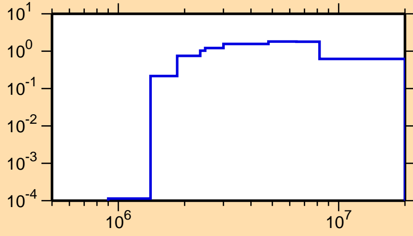
\sigma vs. E for ^{113}\text{Ag}(n,n\text{cont.})
