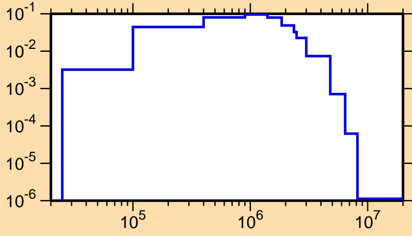
\sigma vs. E for ^{113}\text{Ag}(n,n_1)
