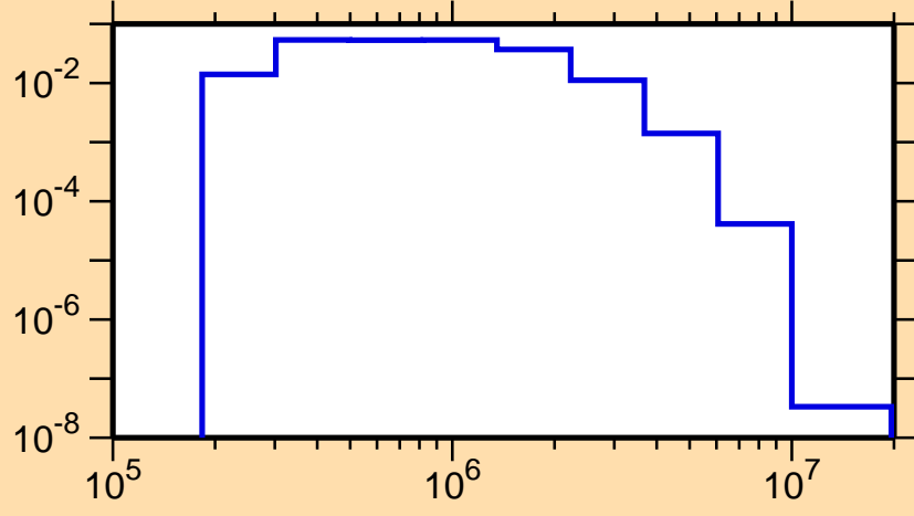
\sigma vs. E for ^{113}\text{Ag}(n,n_4)
