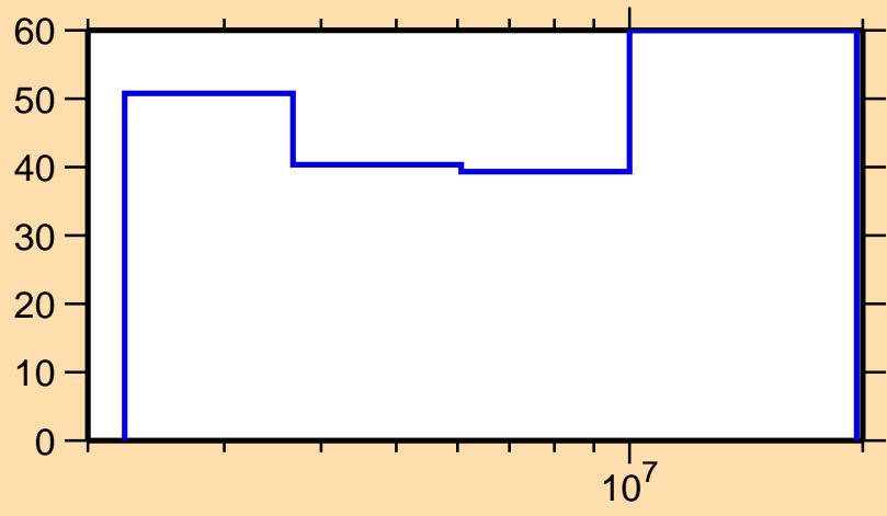
\Delta\sigma/\sigma vs. E for ^{113}\text{Ag}(n,\gamma)
