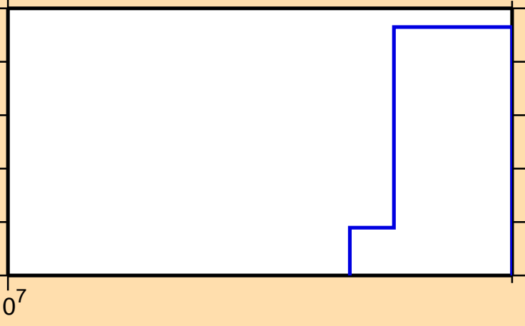
\sigma vs. E for ^{114}\text{Ag}(n,nt)
