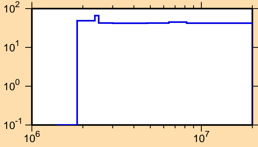
\Delta\sigma/\sigma vs. E for ^{114}\text{Ag}(n,p)
