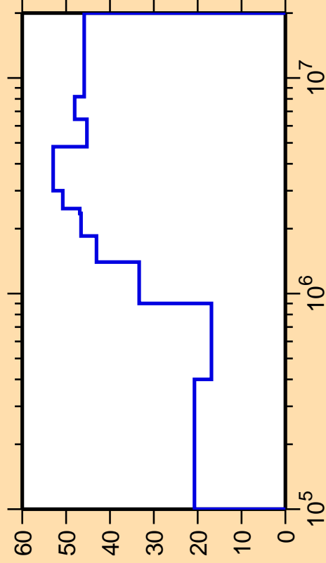
\Delta\sigma/\sigma vs. E for ^{114}\text{Ag}(n,n_4)
