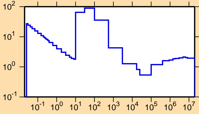
\sigma vs. E for ^{116}\text{Ag}(n,\text{nonel.})
