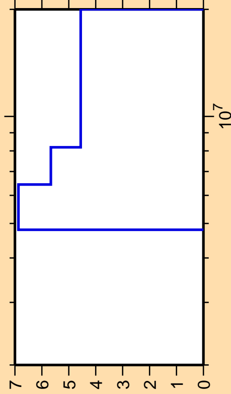
\Delta\sigma/\sigma vs. E for ^{116}\text{Ag}(n,2n)
