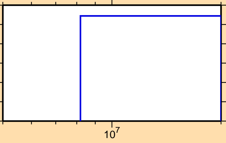
\sigma vs. E for ^{116}\text{Ag}(n,n\alpha)
