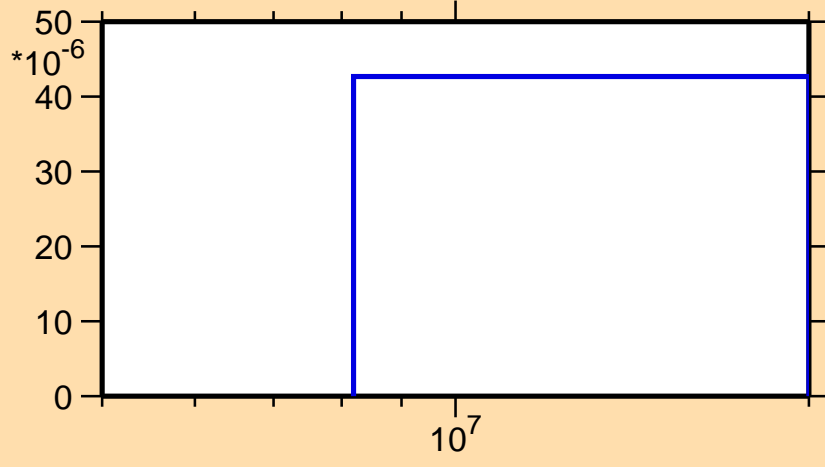
\sigma vs. E for ^{116}\text{Ag}(n,t)
