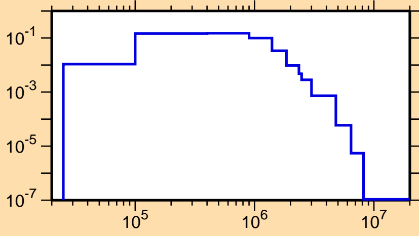
\sigma vs. E for ^{116}\text{Ag}(n,n_3)
