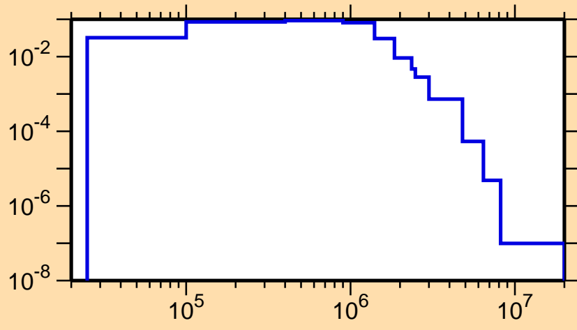
\sigma vs. E for ^{116}\text{Ag}(n,n_2)
