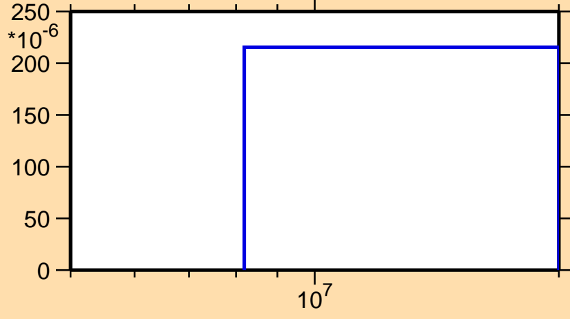
\sigma vs. E for ^{116}\text{Ag}(n,d)
