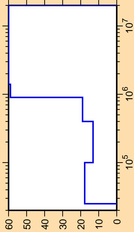
\Delta\sigma/\sigma vs. E for ^{116}\text{Ag}(n,n_2)
