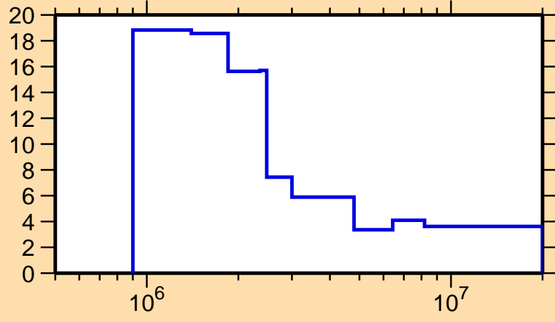
\Delta\sigma/\sigma vs. E for ^{116}\text{Ag}(n,n\text{onel.})
