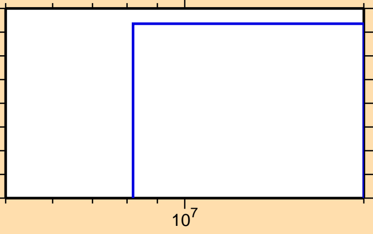
\sigma vs. E for ^{116}\text{Ag}(n,3n)
