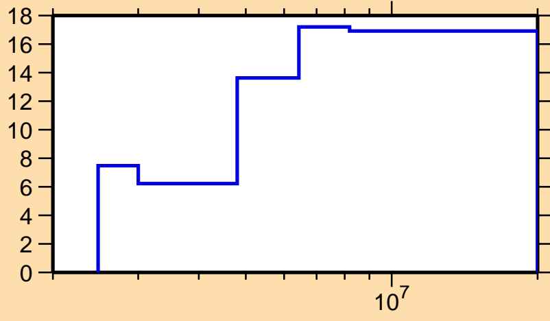
\Delta\sigma/\sigma vs. E for ^{116}\text{Ag}(n,n\text{cont.})
