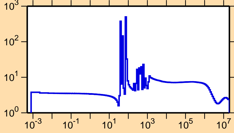
\sigma vs. E for ^{117}\text{Ag}(n,\text{el.})
