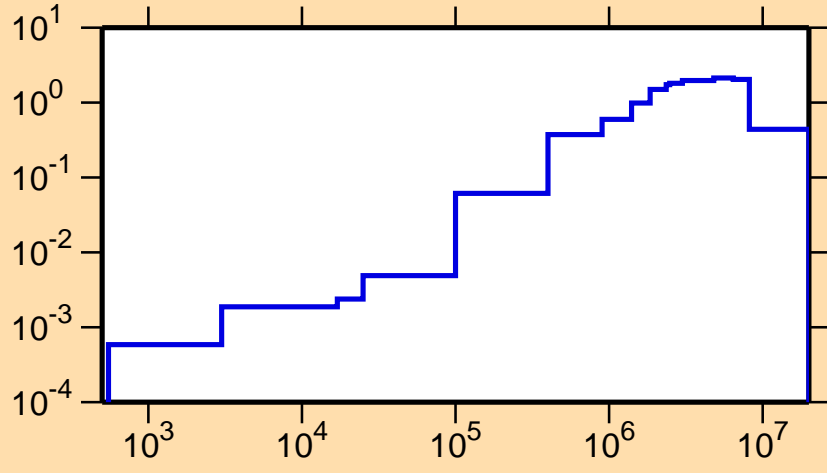
\sigma vs. E for ^{117}\text{Ag}(n,\text{inel.})
