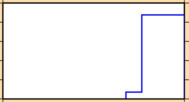
\sigma vs. E for ^{118}\text{Ag}(n,nt)
