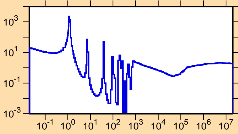
\sigma vs. E for ^{118}\text{Ag}(n,\text{nonel.})
