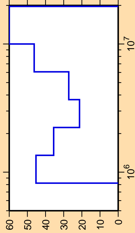
\Delta\sigma/\sigma vs. E for ^{118}\text{Ag}(n,ncont.)
