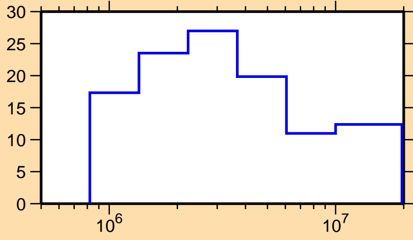
\Delta\sigma/\sigma vs. E for ^{118}\text{Ag}(n,el.)
