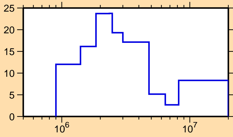
\Delta\sigma/\sigma vs. E for ^{118}\text{Ag}(n,\text{tot.})
