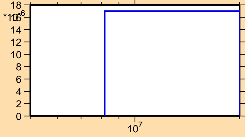
\sigma vs. E for ^{118}\text{Ag}(n,t)
