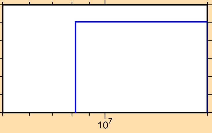
\sigma vs. E for ^{118}\text{Ag}(n,2np)
