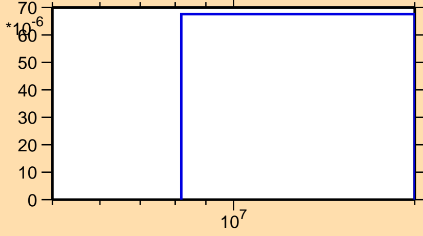
\sigma vs. E for ^{118}\text{Ag}(n,d)
