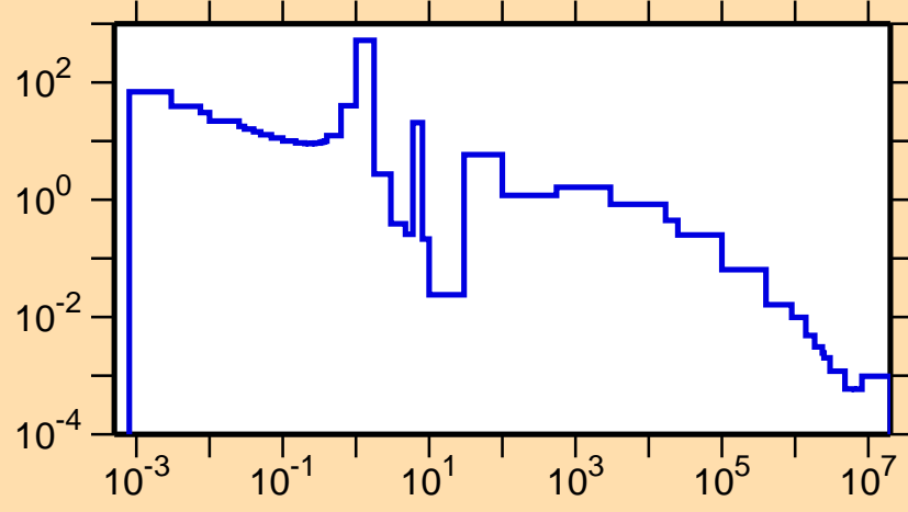
\sigma vs. E for ^{118}\text{Ag}(n,\gamma)
