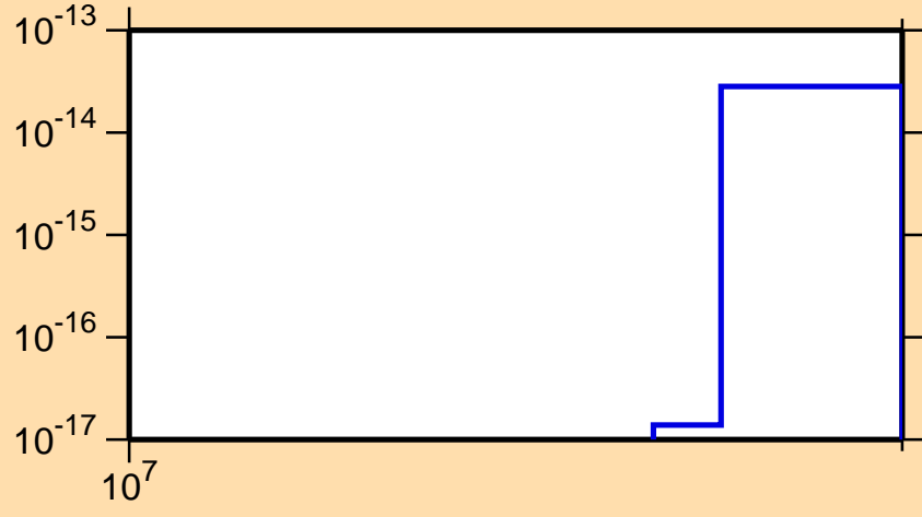
\sigma vs. E for ^{119}\text{Ag}(n,2n\alpha)
