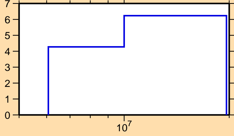
\Delta\sigma/\sigma vs. E for ^{119}\text{Ag}(n,\text{tot.})
