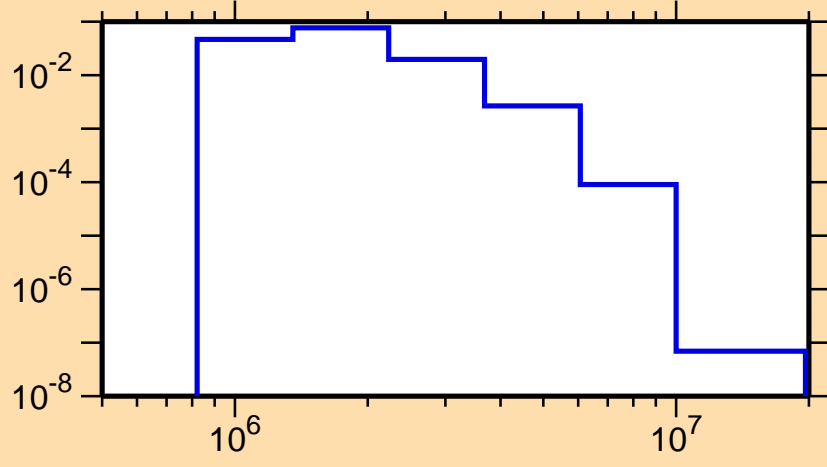
\sigma vs. E for ^{119}\text{Ag}(n,n_4)
