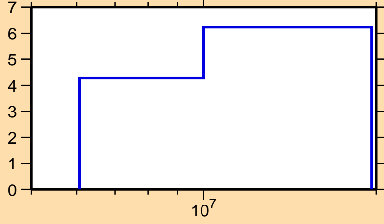
\Delta\sigma/\sigma vs. E for ^{119}\text{Ag}(n,\text{tot.})
