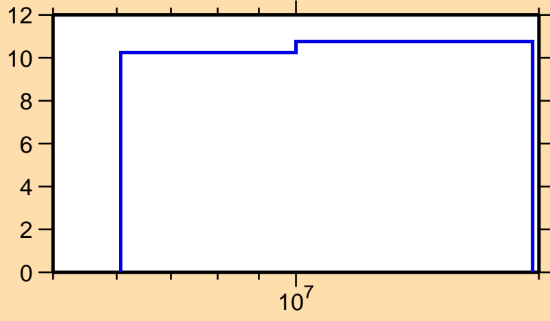
\Delta\sigma/\sigma vs. E for ^{119}\text{Ag}(n,el.)
