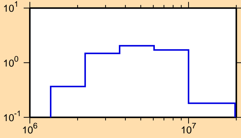
\sigma vs. E for ^{119}\text{Ag}(n,n\text{cont.})
