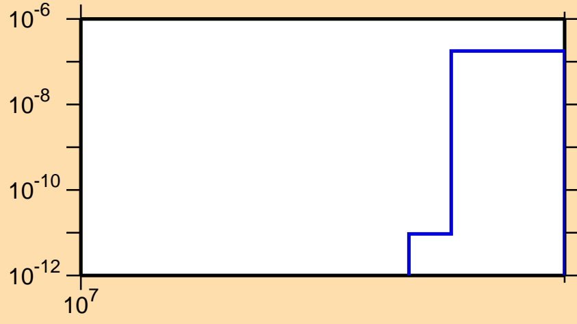
\sigma vs. E for ^{120}\text{Ag}(n,nt)
