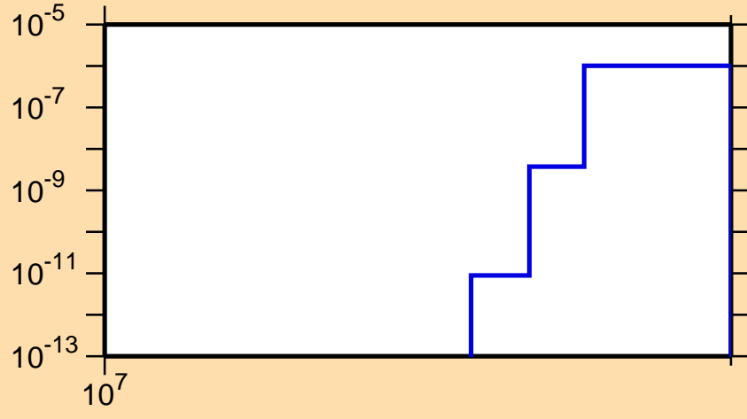
\sigma vs. E for ^{120}\text{Ag}(n,\text{nd})
