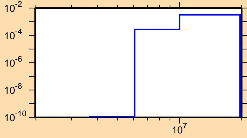
\sigma vs. E for ^{30}\text{Al}(n,\alpha)
