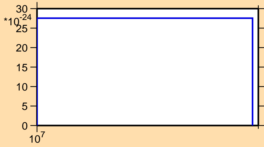
\sigma vs. E for ^{30}\text{Al}(n,p\alpha)
