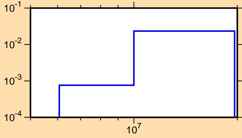
\sigma vs. E for ^{30}\text{Al}(n,p)
