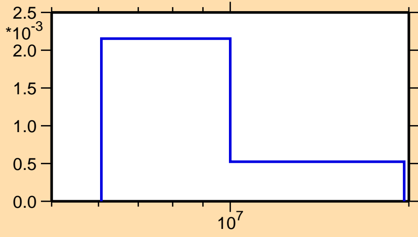
\sigma vs. E for ^{30}\text{Al}(n,n\text{cont.})
