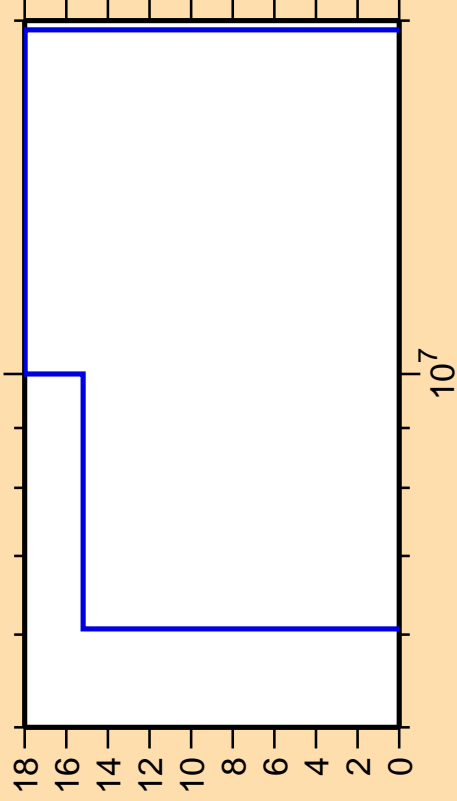
\Delta\sigma/\sigma vs. E for ^{30}\text{Al}(n,t)
