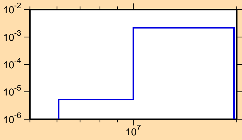
\sigma vs. E for ^{30}\text{Al}(n,t)
