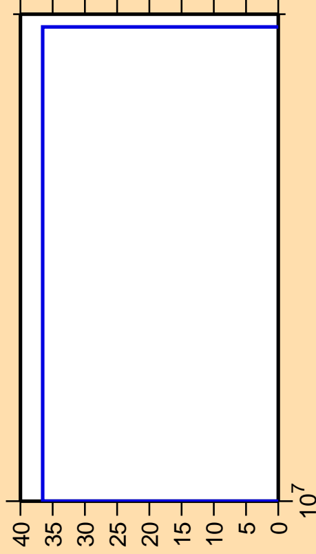
\Delta\sigma/\sigma vs. E for ^{30}\text{Al}(n,\text{nd})
