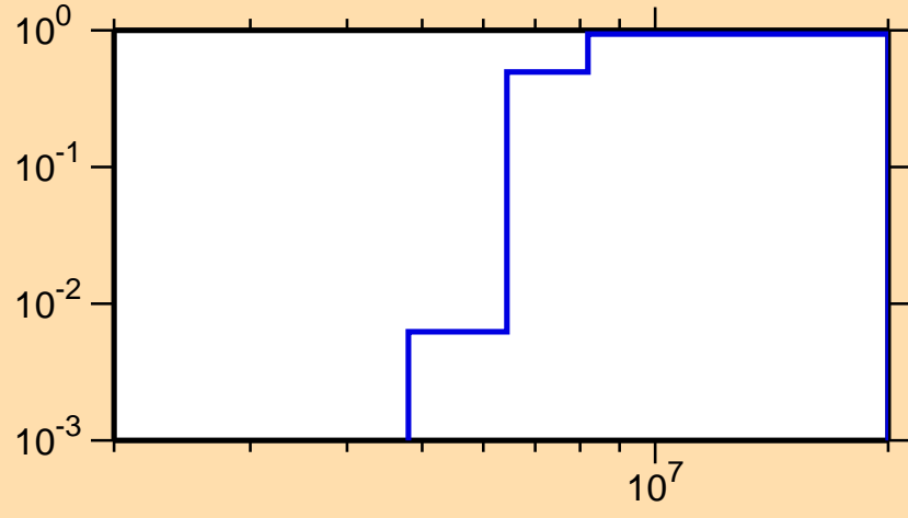
\sigma vs. E for ^{30}\text{Al}(n,2n)
