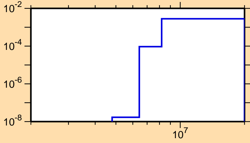
\sigma vs. E for ^{30}\text{Al}(n,\alpha)
