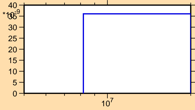
\sigma vs. E for ^{30}\text{Al}(n,2np)
