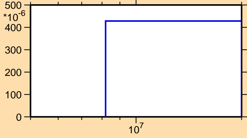
\sigma vs. E for ^{30}\text{Al}(n,3n)
