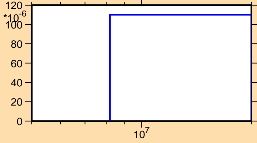
\sigma vs. E for ^{30}\text{Al}(n,n\alpha)
