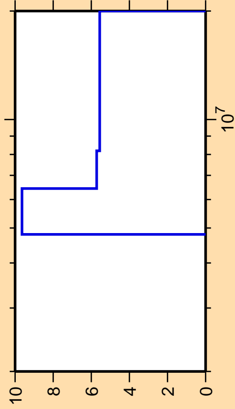
\Delta\sigma/\sigma vs. E for ^{30}\text{Al}(n,2n)
