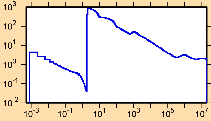
\sigma vs. E for ^{230}\text{Am}(n,f)
