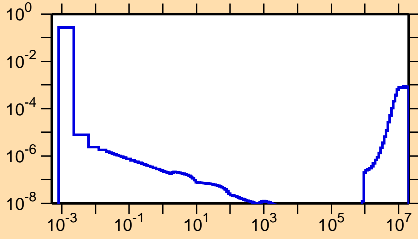
\sigma vs. E for ^{230}\text{Am}(n,\alpha)
