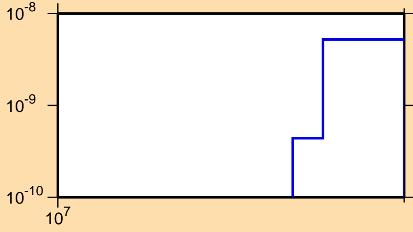
\sigma vs. E for ^{230}\text{Am} (mt 34)
