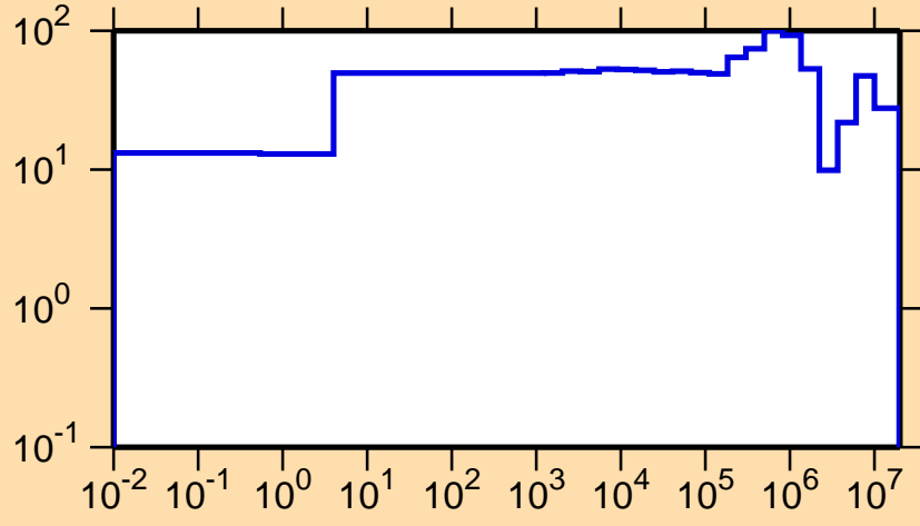
\Delta\sigma/\sigma vs. E for ^{230}\text{Am}(n,el.)
