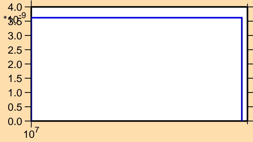
\sigma vs. E for ^{230}\text{Am}(n,3n)
