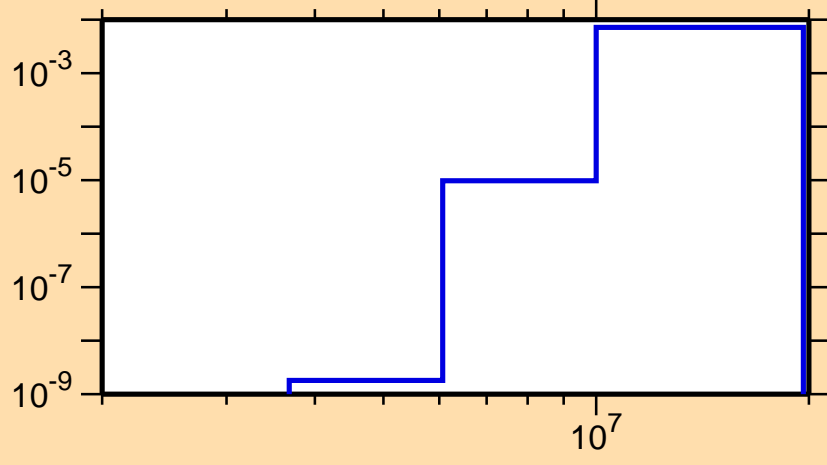
\sigma vs. E for ^{230}\text{Am}(n,d)
