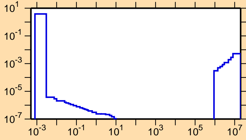
\sigma vs. E for ^{230}\text{Am}(n,p)
