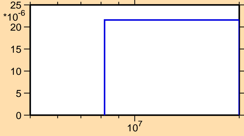
\sigma vs. E for ^{230}\text{Am}(n,\text{nd})
