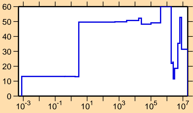
\Delta\sigma/\sigma vs. E for ^{230}\text{Am}(n,el.)
