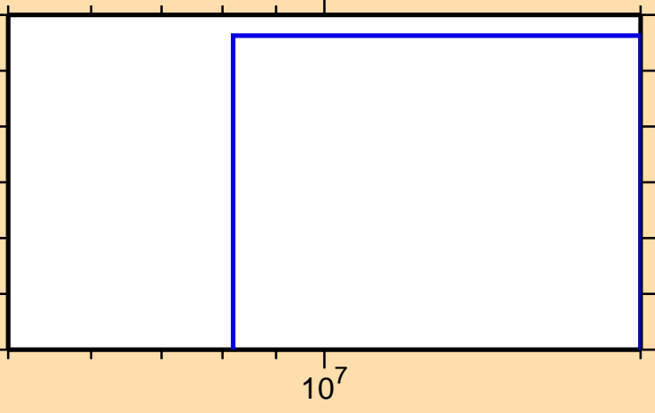
\sigma vs. E for ^{230}\text{Am}(n,3n\alpha)
