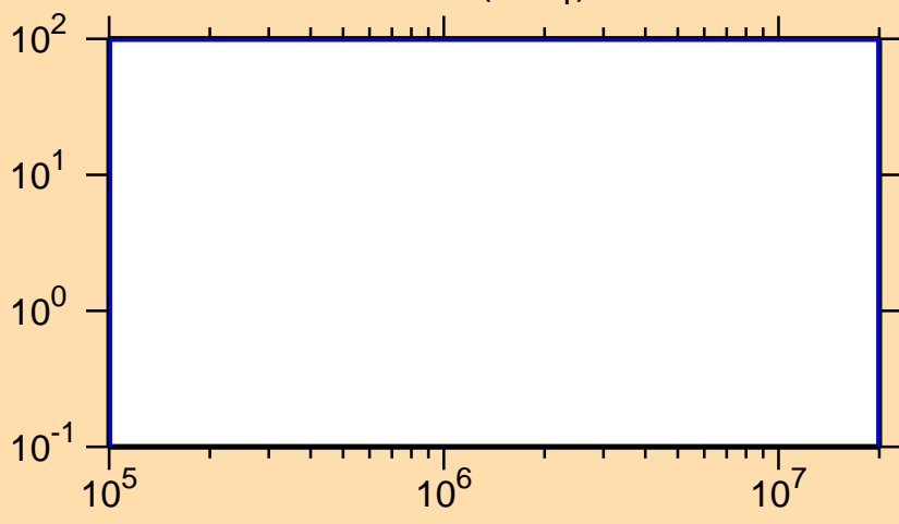
\Delta\sigma/\sigma vs. E for ^{230}\text{Am}(n,n_1)
