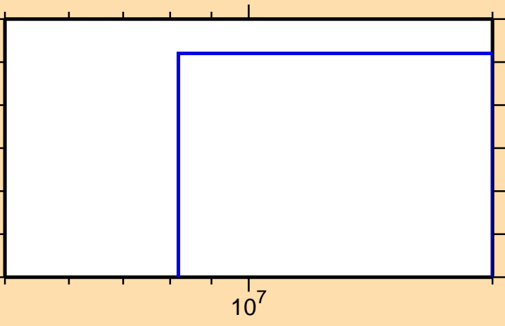
\sigma vs. E for ^{230}\text{Am} (mt 45)
