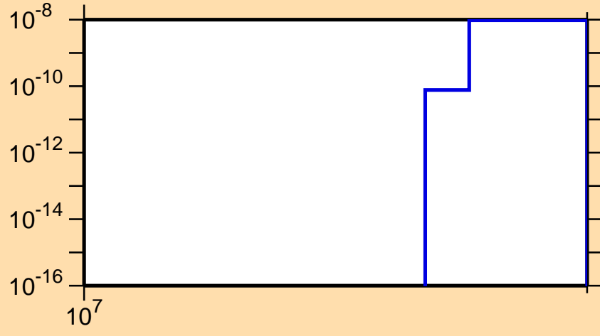
\sigma vs. E for ^{231}\text{Am}(n,3n)
