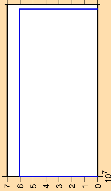
\Delta\sigma/\sigma vs. E for ^{231}\text{Am}(n,3n\alpha)
