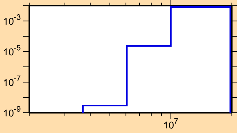
\sigma vs. E for ^{231}\text{Am}(n,d)
