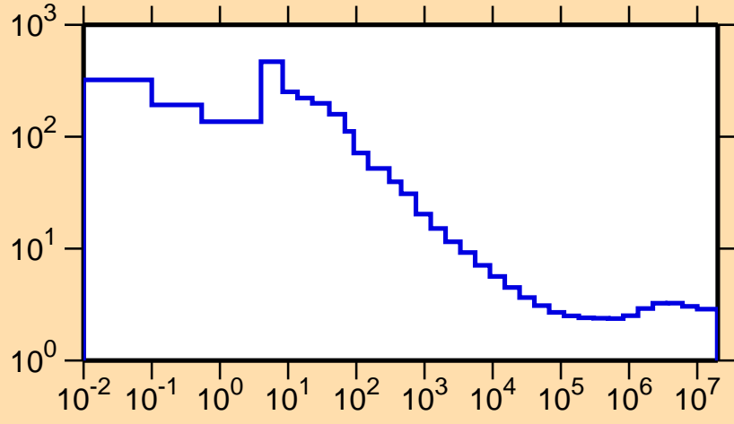
\sigma vs. E for ^{231}\text{Am}(n,\text{nonel.})
