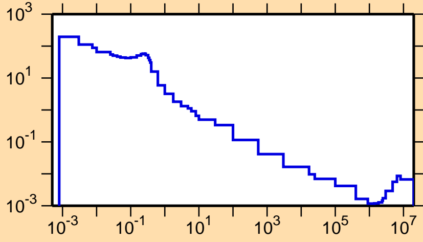
\sigma vs. E for ^{231}\text{Am}(n,\gamma)
