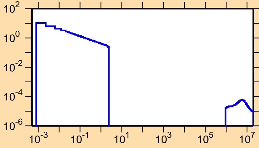
\sigma vs. E for ^{232}\text{Am}(n,\gamma)
