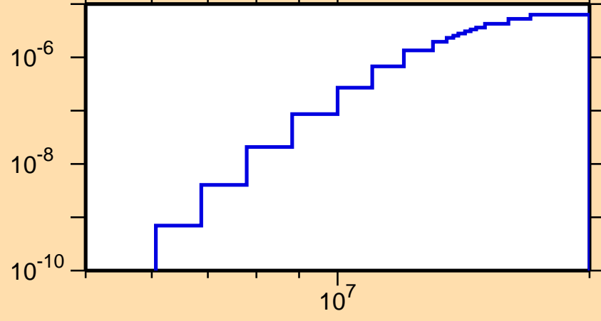
\sigma vs. E for ^{232}\text{Am}(n,p\alpha)
