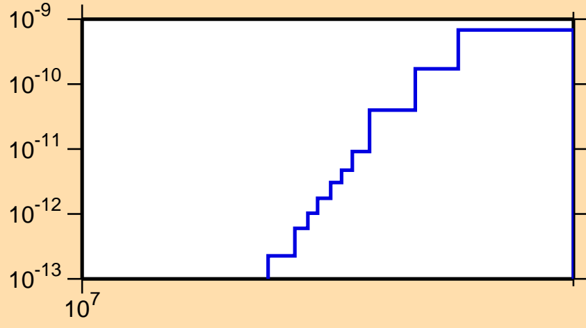
\sigma vs. E for ^{232}\text{Am}(n,\text{nd})
