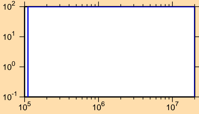
\Delta\sigma/\sigma vs. E for ^{232}\text{Am}(n,ncont.)
