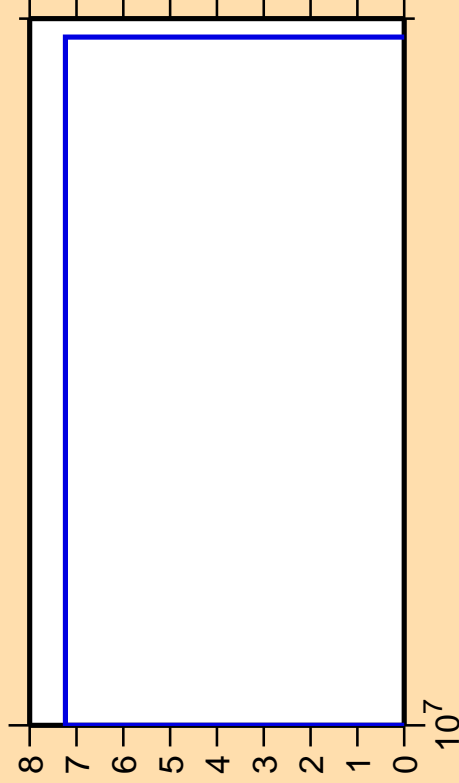
\Delta\sigma/\sigma vs. E for ^{232}\text{Am} (mt 45)
